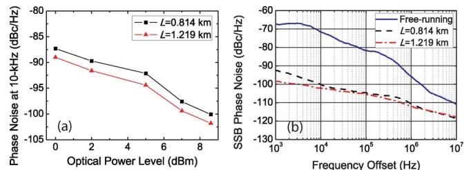
Fig. 3. (a) RTD-OEO SSB phase noise at 10 kHz as a function of in-fiber optical power for L = 0.814 km and L = 1.219 km. (b) Measured SSB phase noises (smoothed traces) for P \sim 8.6 dBm and free-running oscillation.
