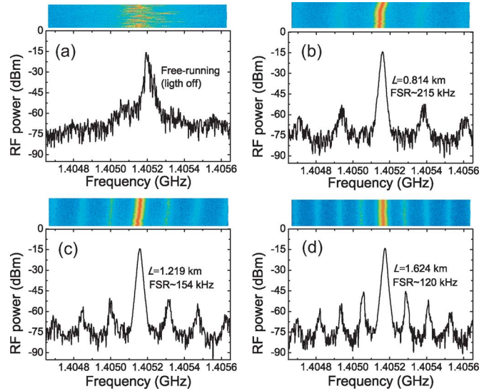
Fig. 2. RF power spectrum traces of the RTD-OEO output. (a) Free-running. Self-synchronization at P \sim 5 dBm using fiber loops of (b) L = 0.814 km, (c) L = 1.219 km, and (d) L = 1.624 km. The frequency span and resolution bandwidth settings of all figures were 1 MHz and 10 kHz, respectively. The top part of each figure shows a spectrogram that represents the evolution of spectral density recorded over \sim 30 s.
