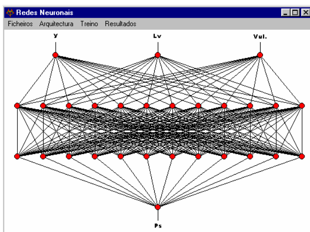
FIGURA 6 - Rede neuronal Multilayer Feedforward .
